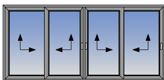
Four lifting sliding sashes meeting stile
